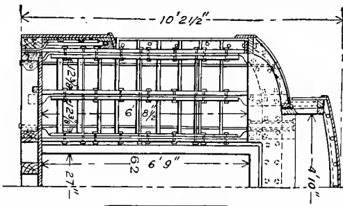
Fig. 523-526. CAR-BODIES, Passenger; Framing for Sleeping Cars.
